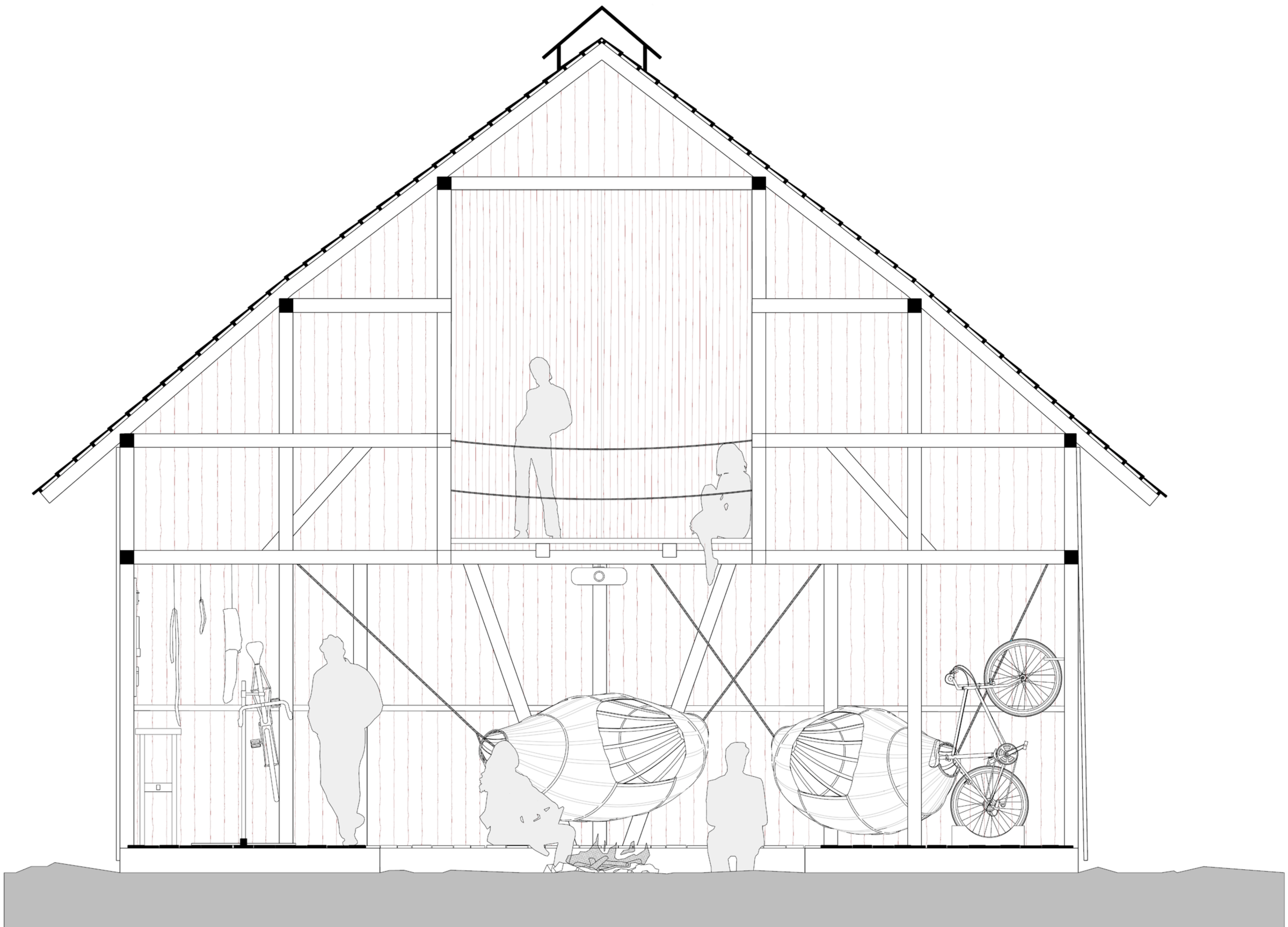
Section 1:20
