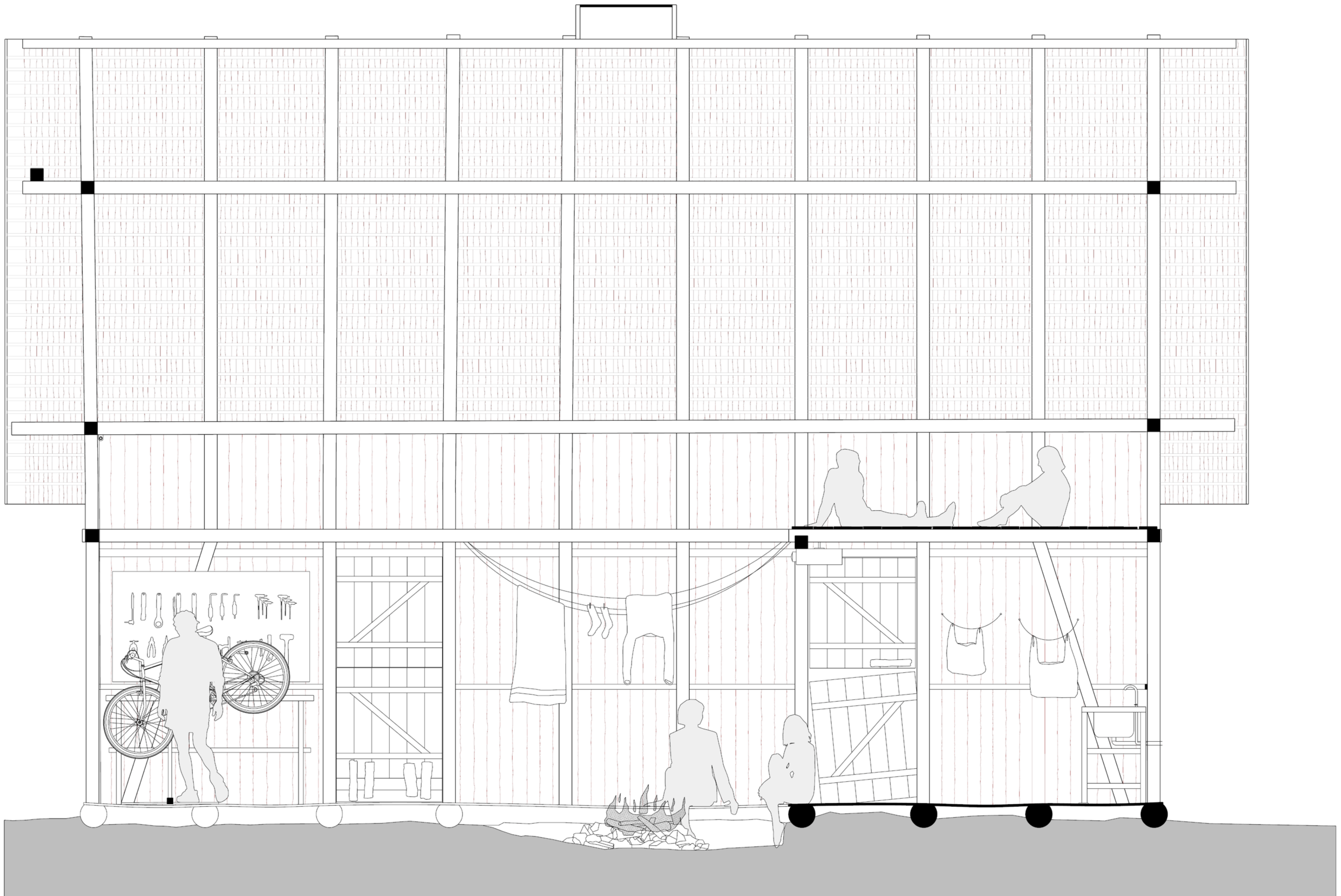
Section 1:20
