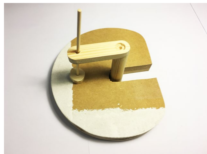
The size of the base is 200mm diameter, I tried 300 diameter as the floor lamp version. The base is too big, too dominant, so that in the end the dimension of the base is 200mm*20mm, if it made in steel it can offer more than 5kg weight, which is enough for the floor lamp.
