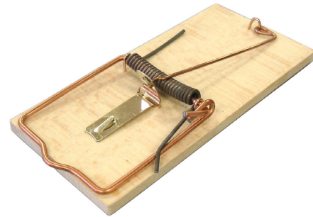
The classic wooden spring trap. It is cheap and often does the trick but it feels unsafe to handle and the open design means more cases of misfire causing a crippled rat instead of a dead one.
