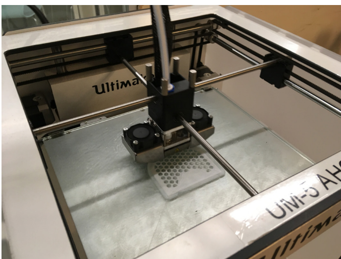
3D printing the bait drawer on the Ultimaker.
