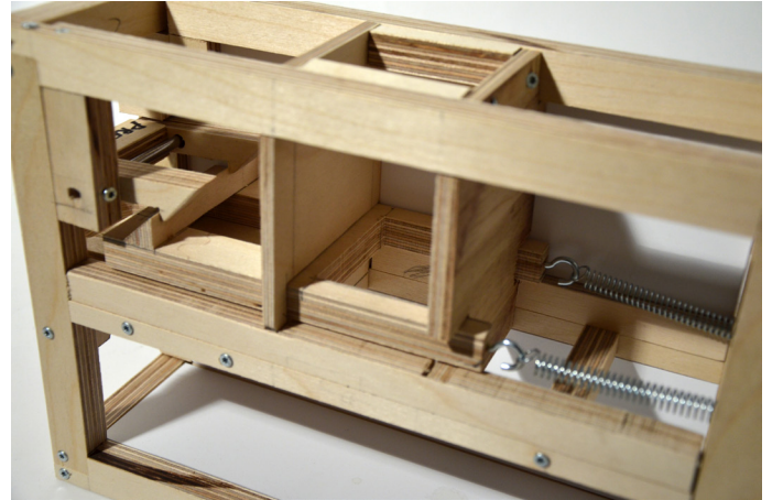
To the right we can see the springs which pulls the bar shut. They are attached in the opposite end from the handle.
