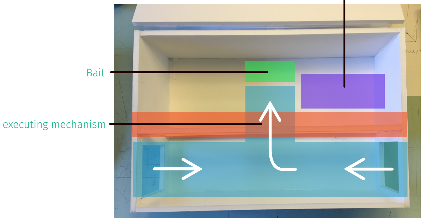
Basic schematics of the layout. The blue shows the t-shaped tunnel with two openings and the bait enclosed in the middle. The trap springs when the rat pokes its head up towards the bait.
