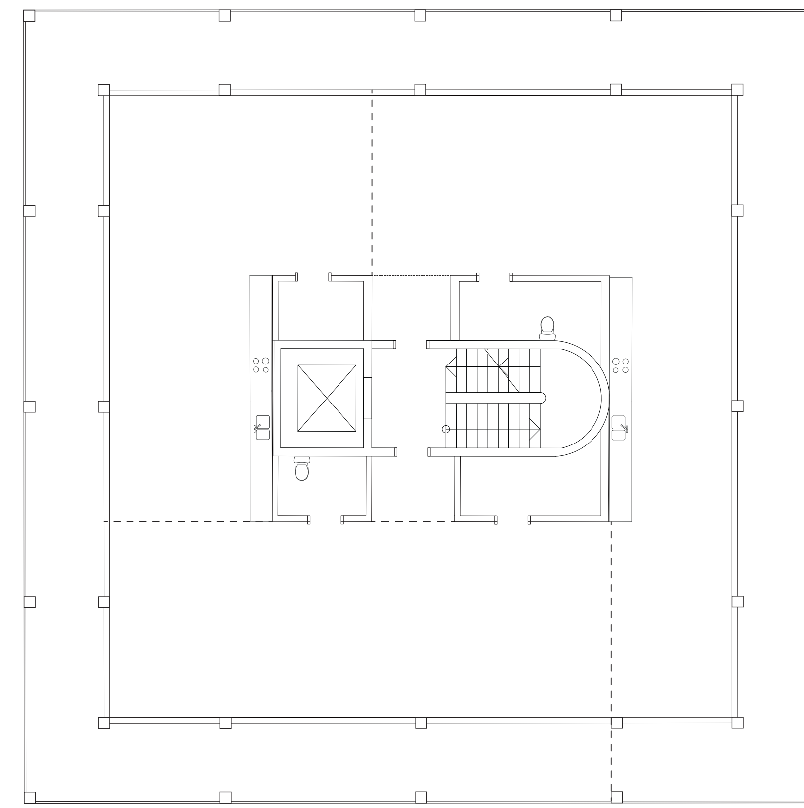
Tower plan with a core with vertical communication, toilets and kitchens. Frees up space for the inhabitants to decide for them self how to build a floor. Outside terrace connecting the floors together.
