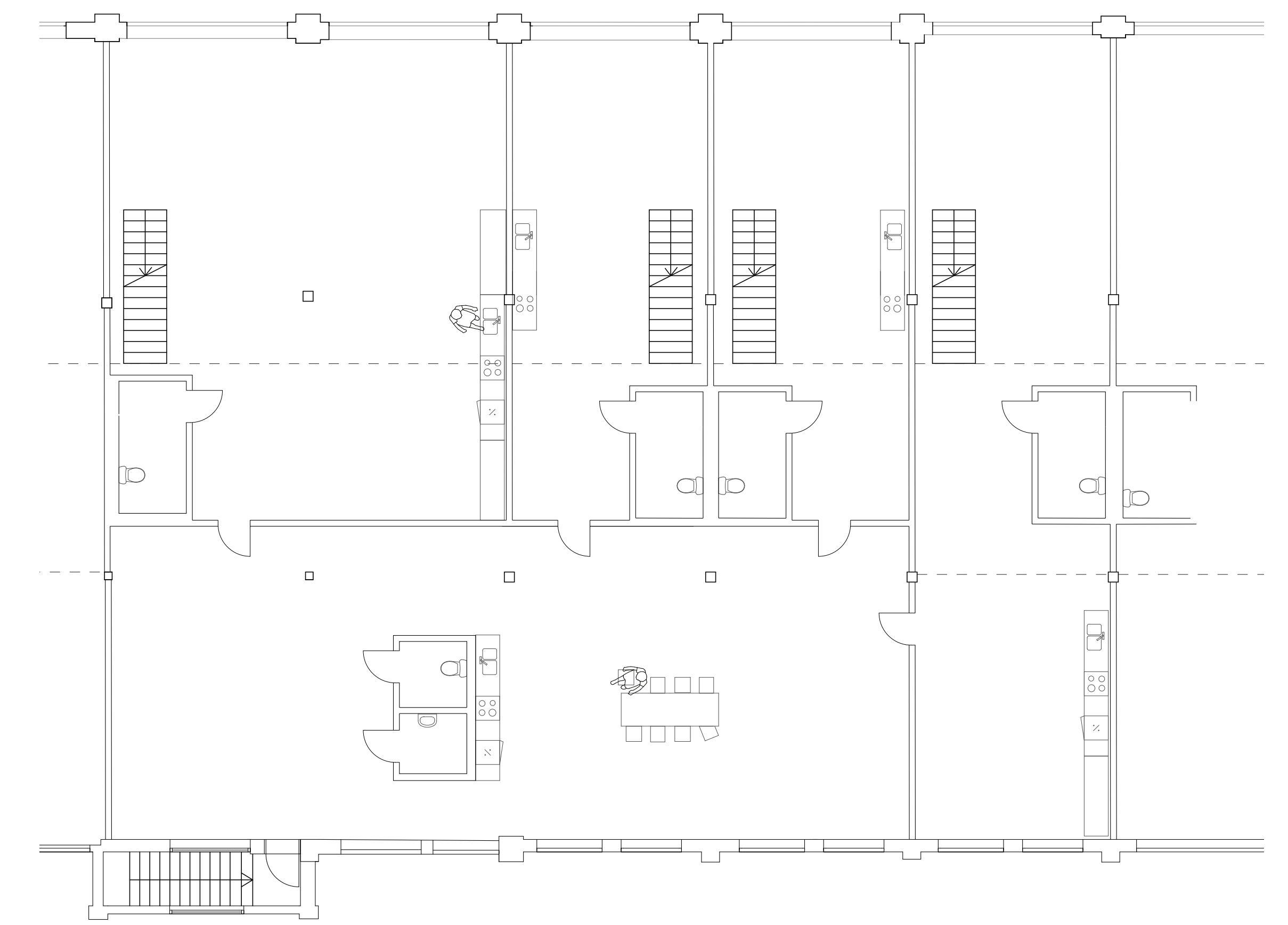
Private small apartments with gallery for sleeping upstairs. Access to common rooms form all the apartments.
