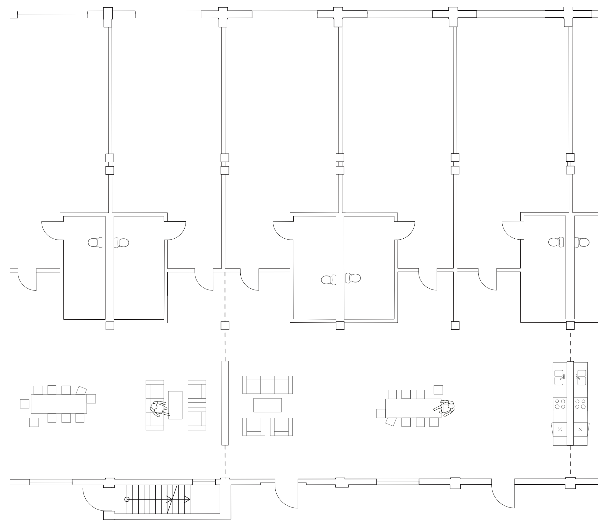
Spacious private rooms with bathrooms. Shares kitchen and living area. Possible to move between the common rooms.
