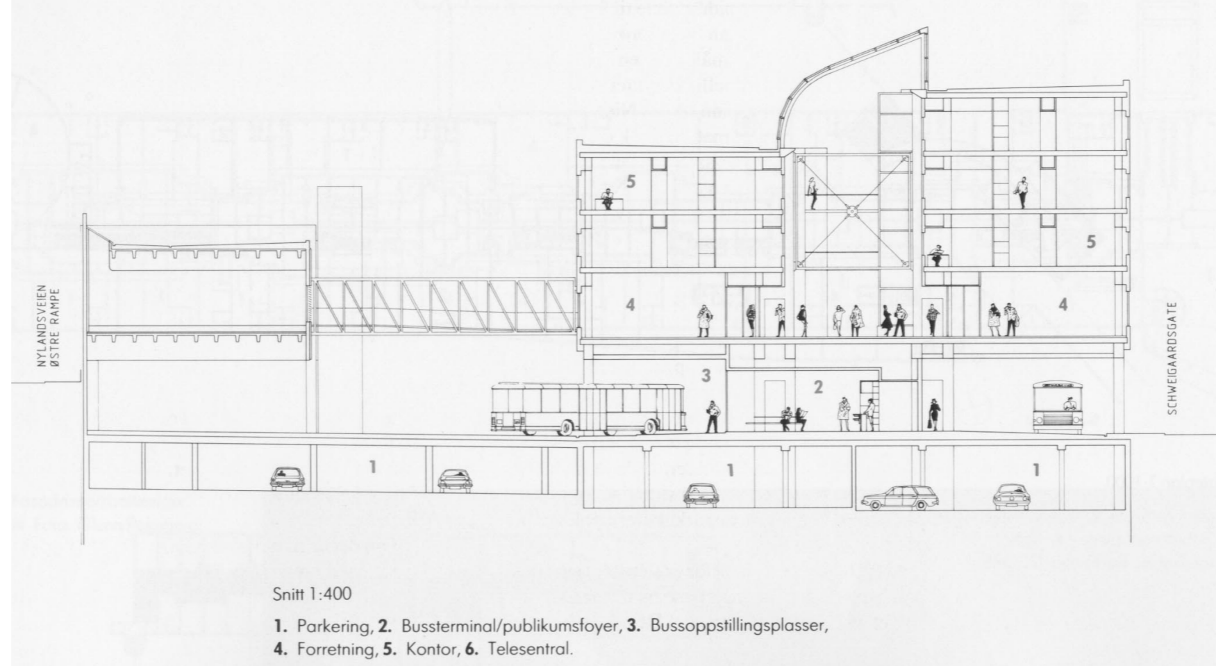
Section through main building and telecom switchboard centre
