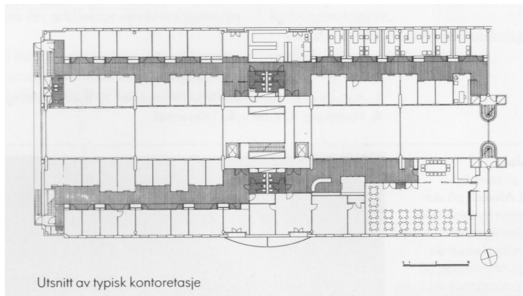
Typical office plan
