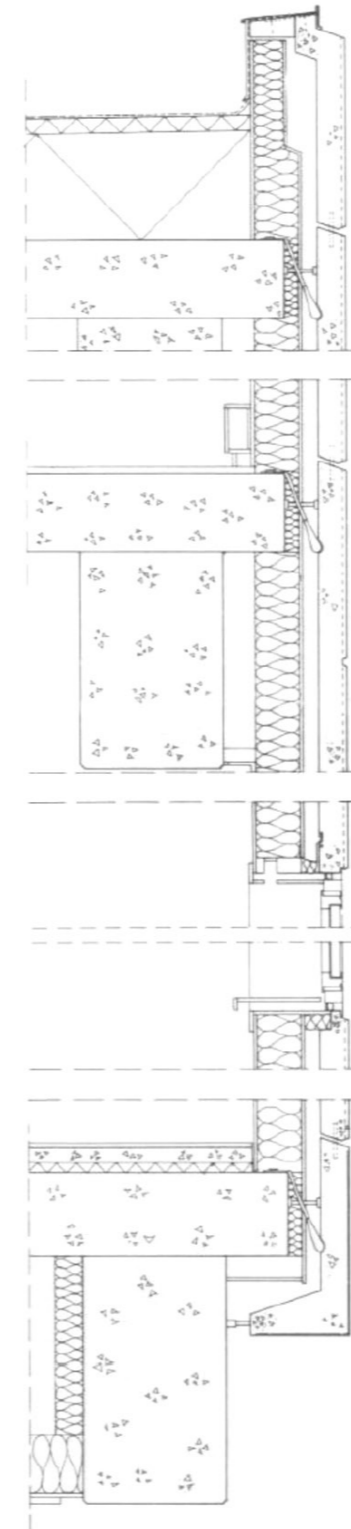
Section through facade element
