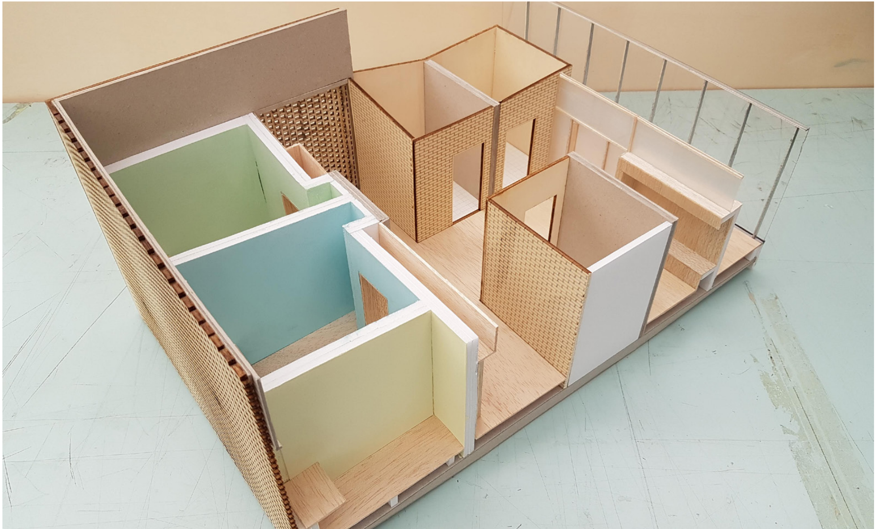
user rooms on the left, toilets and user wardrobe in the middle, circulation hallway on the right
