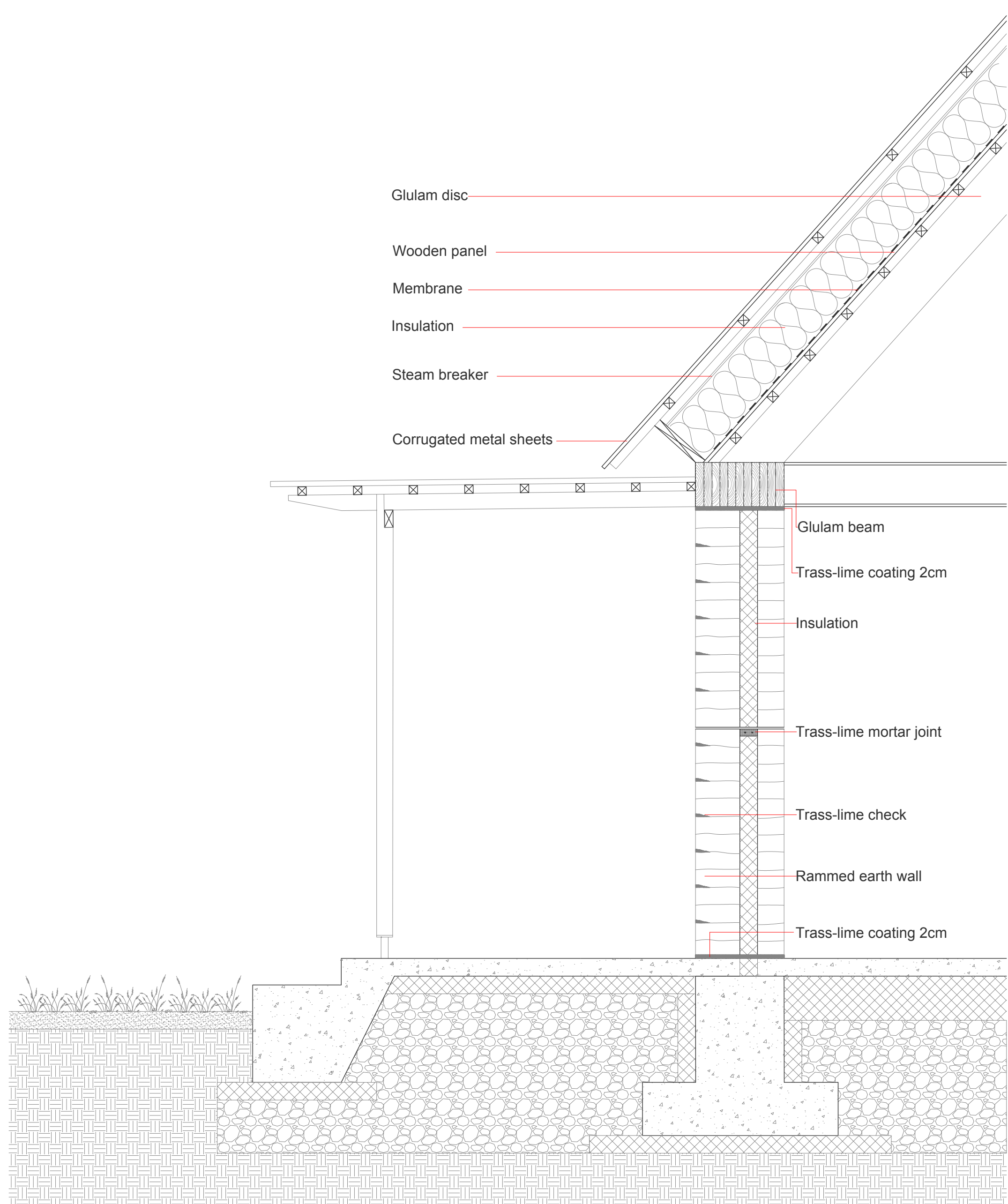
Detail section
