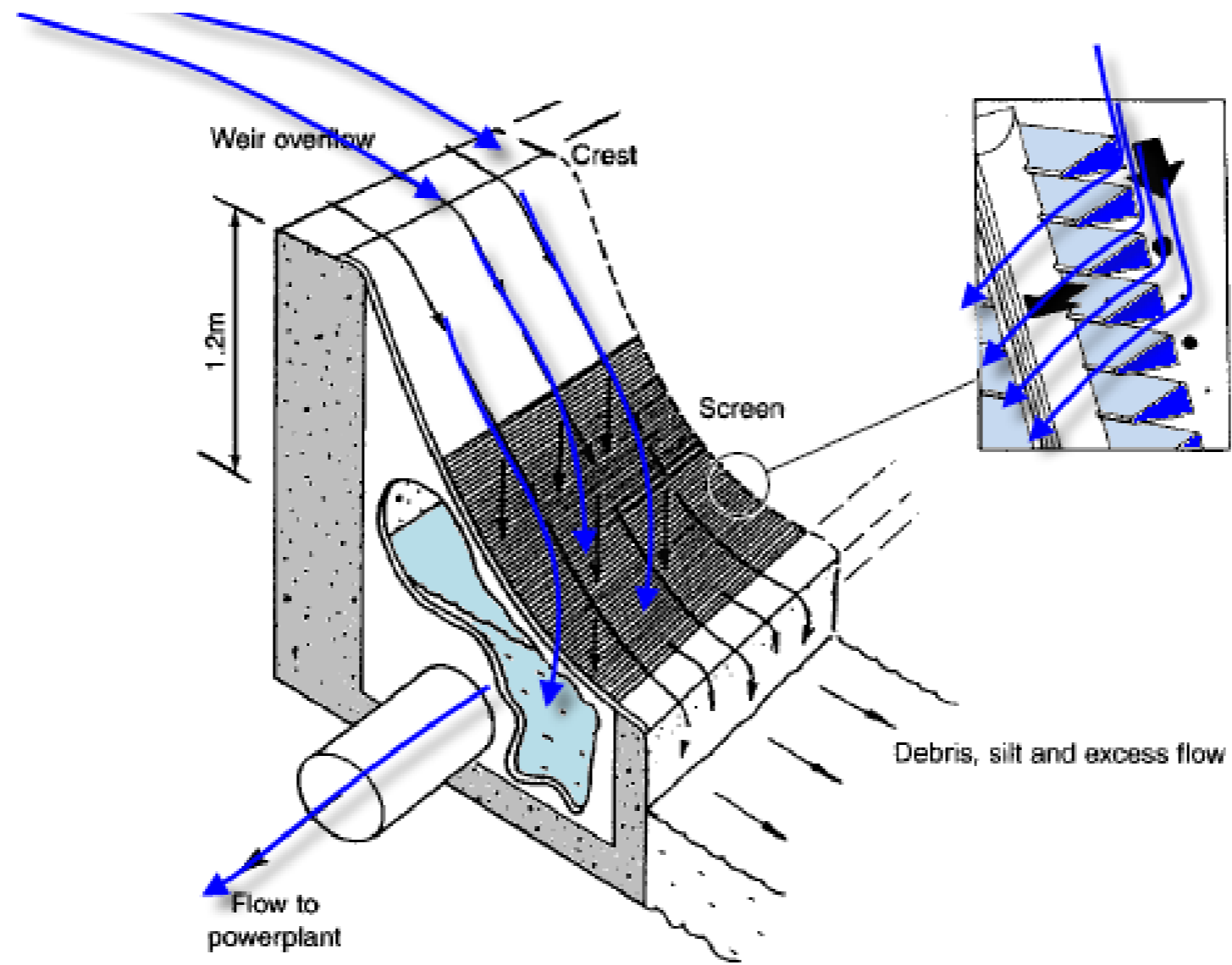
– Schematic of Coanda Effect Screen
