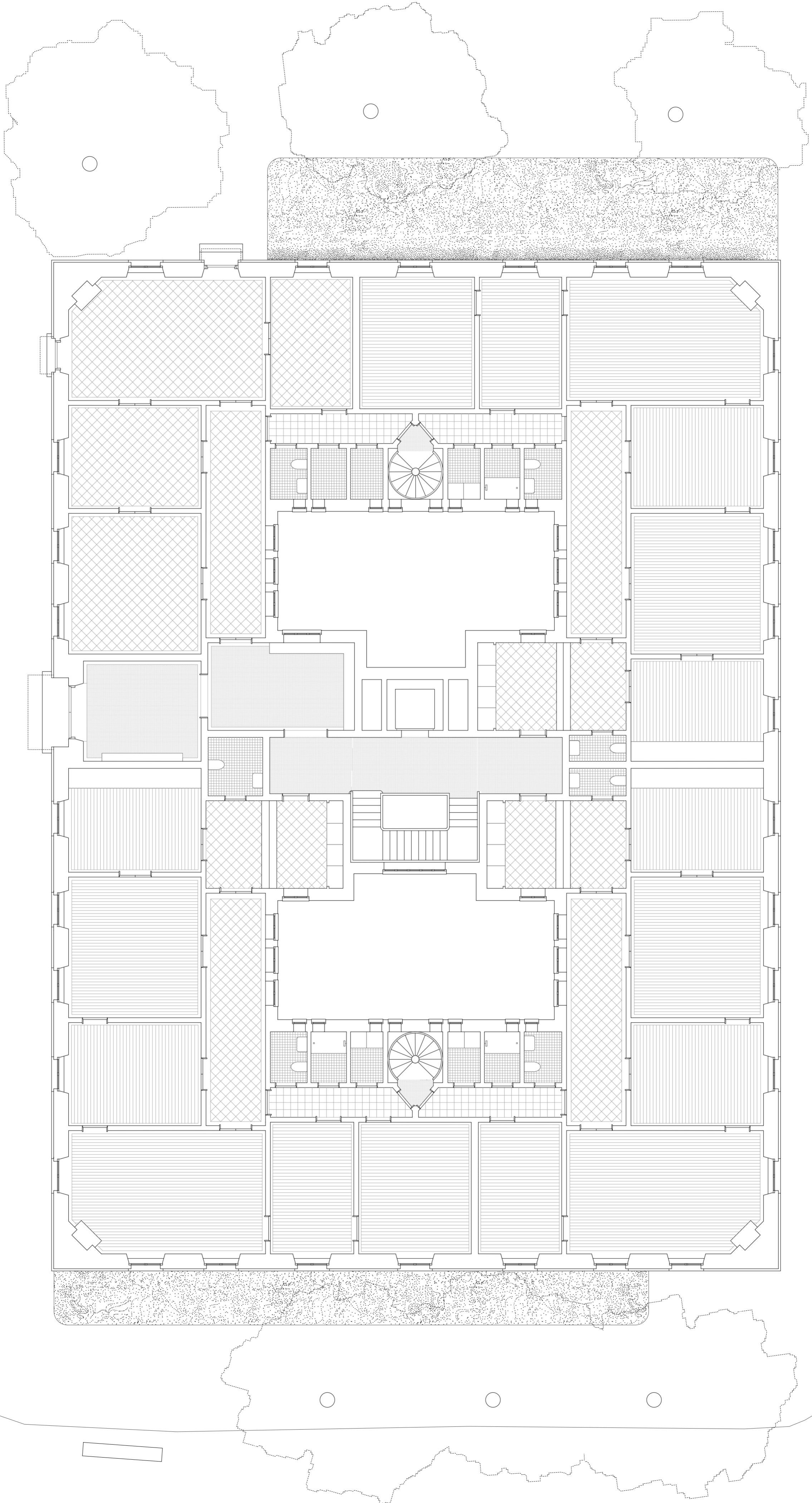
Ground floor 1:100
