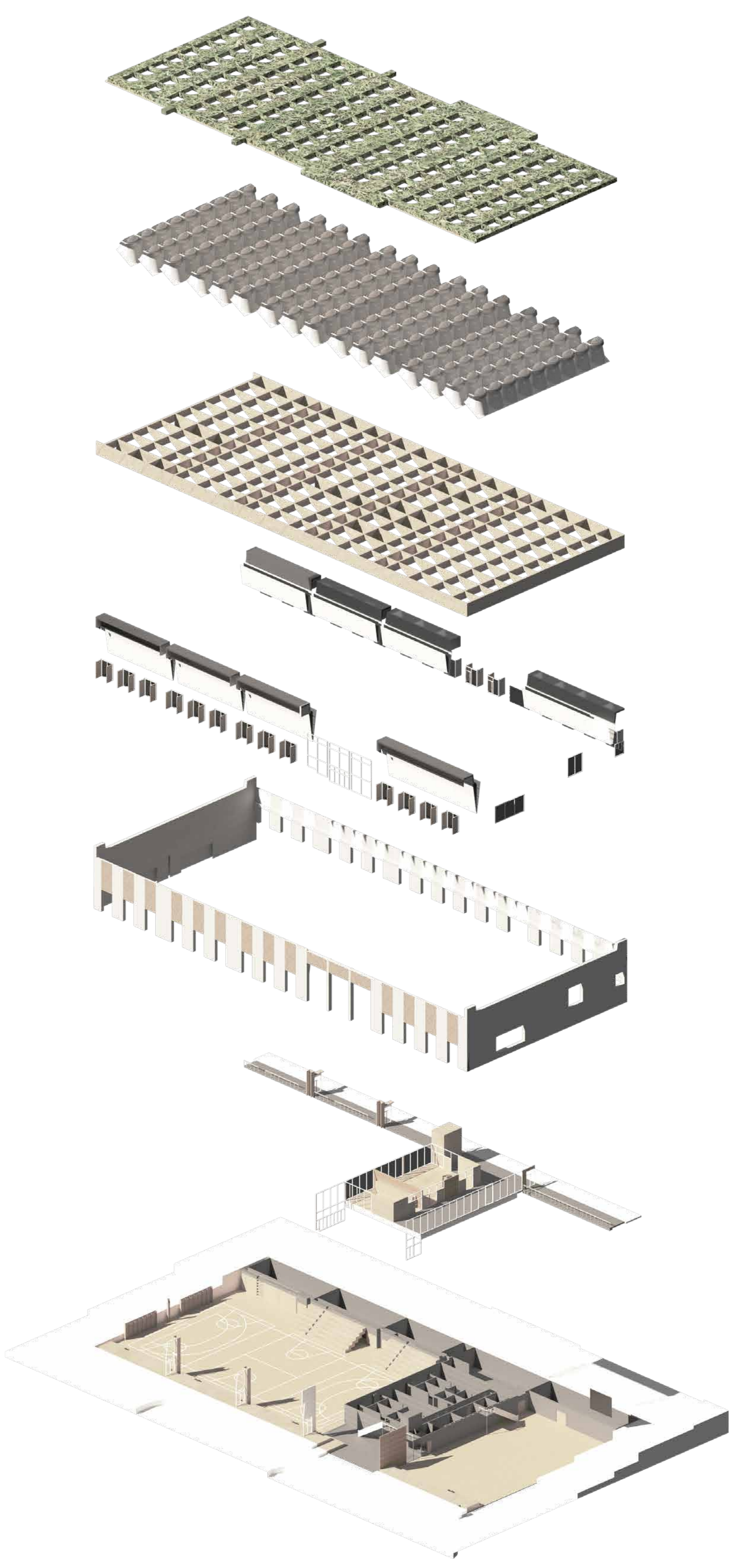
Axonometric representation of the project elements
