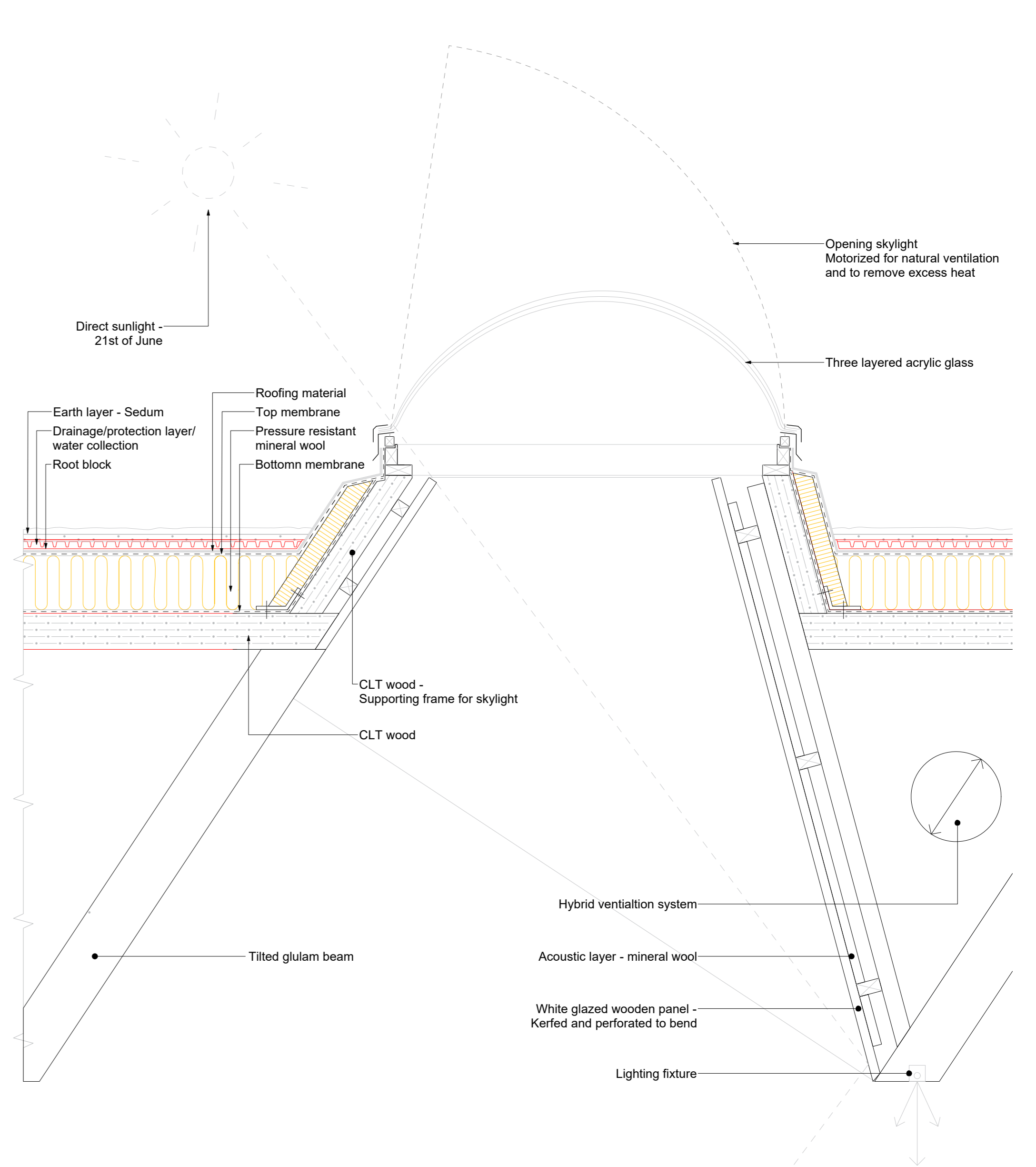
Skylight detail Scale 1:20
