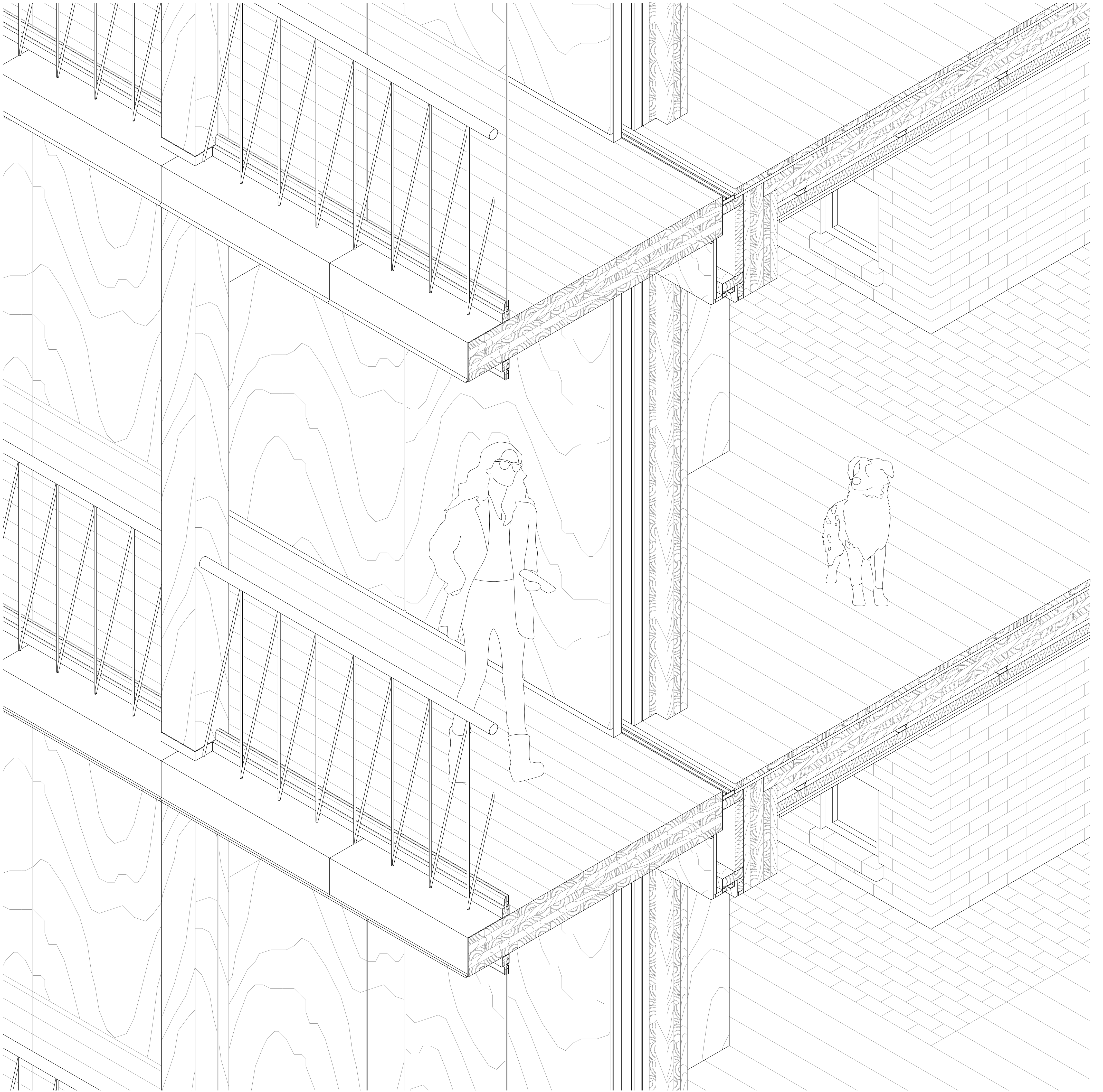
DETAIL 1:10
